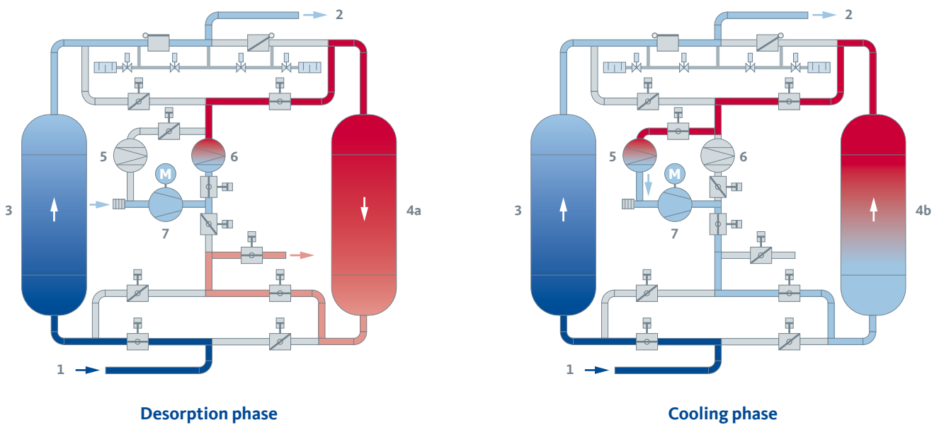
(1) Moist air inlet (2) Dry air outlet (3) Vessel in adsorption mode (4a) Vessel in desorption mode (4b) Vessel in cooling mode (5) Cooler (6) Heater (7) Fan
